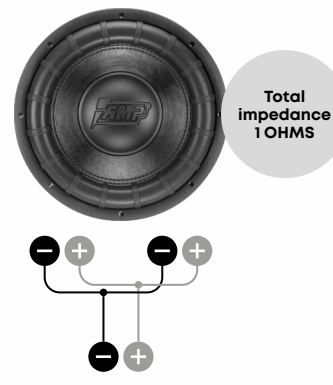
Subwoofers in parallel, coils in parallel
